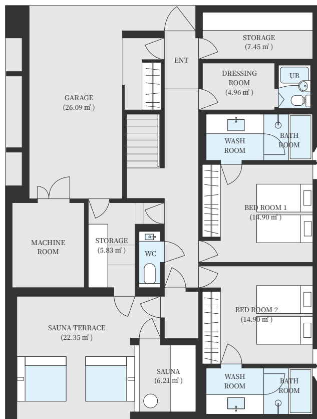
1F Plan
