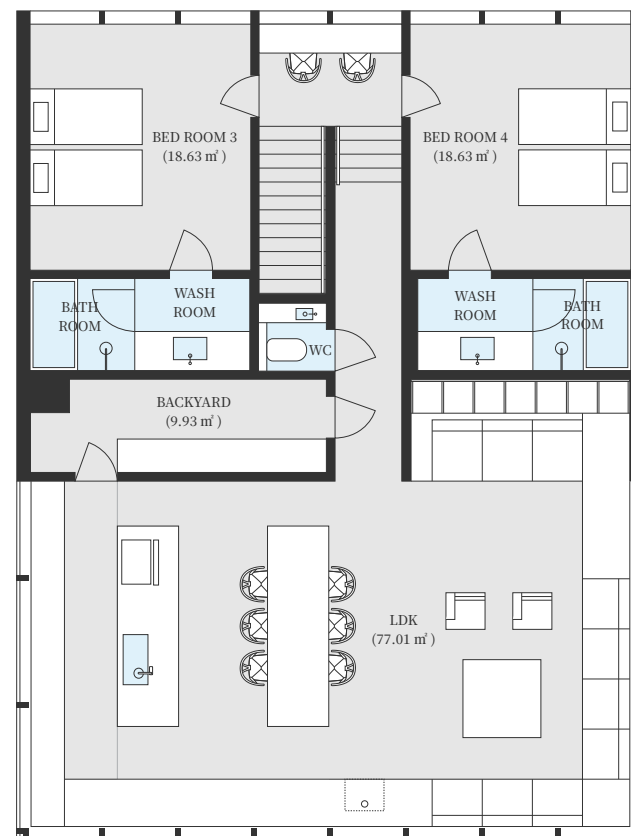
2F Plan
