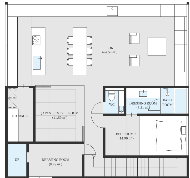
2F Plan
